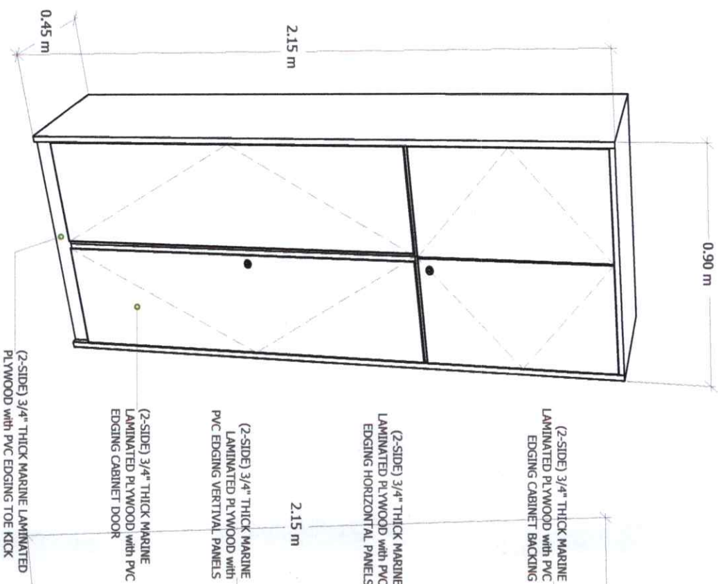
ISOMETRIC DRAWING OUTER PARTITION
