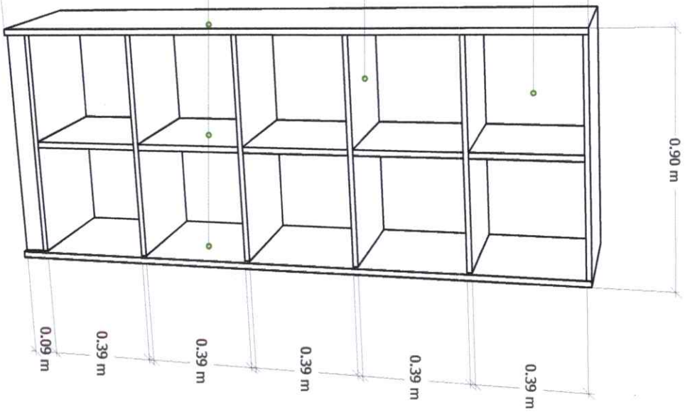
ISOMETRIC DRAWING INNER PARTITION
